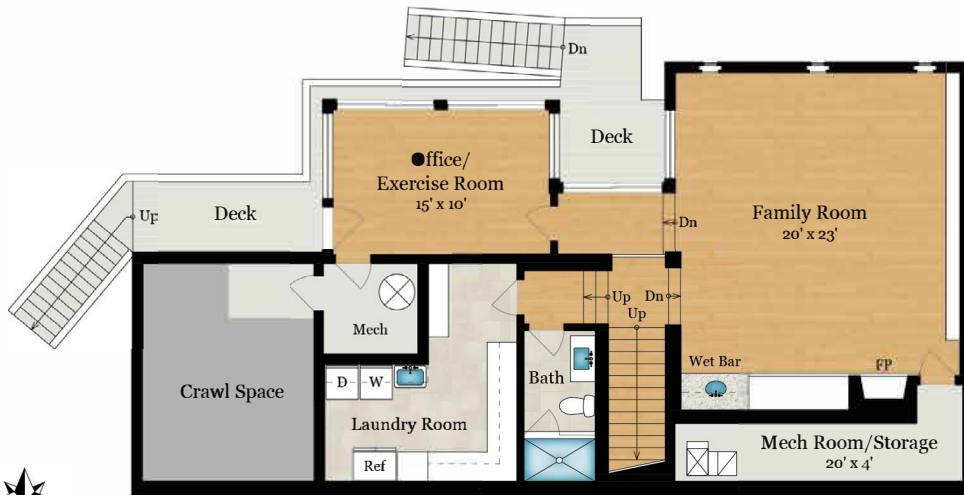
MAIN RESIDENCE LOWER LEVEL 2 1,105 SQ FT
