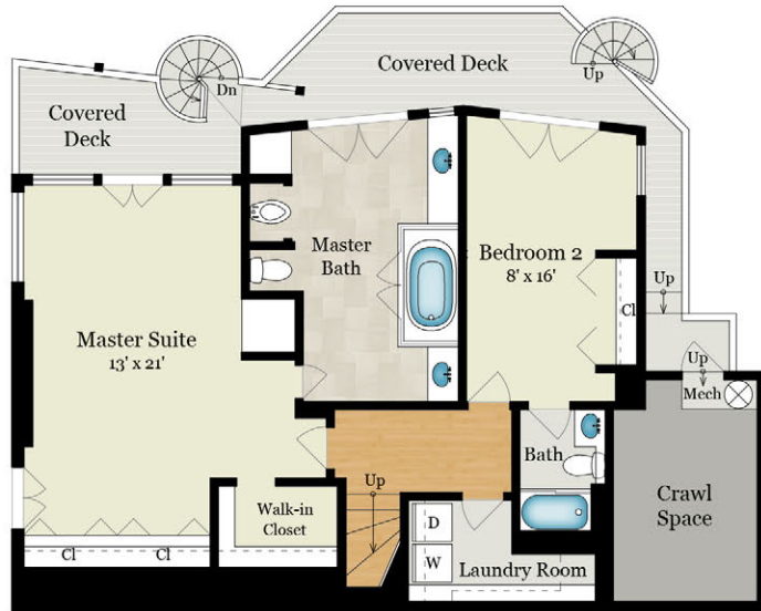
MAIN RESIDENCE LOWER LEVEL 2
